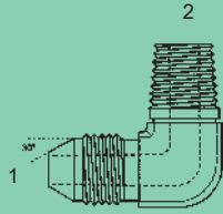
JISBP-BST-2501 - 90° (1) Male 30° BPP (Flare) (2) Male BSPT
