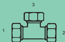
MFL-2603 - Tee (1) (2) (3) Male Flareless Light
