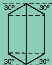
JISBP-0321 JIS Sealing Seat (Converts Male 30° BPP Coneseat To 30° JIS Flare)
