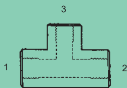
BPP-5605 - Tee (1) (2) (3) Fem. BPP
