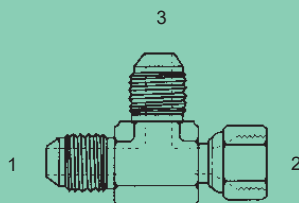
JISM-6602 - Tee (1) (3) Male 30° Metric Komatsu Tee (2) Fem. 30° Metric Komatsu Swivel
