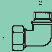
MFL-BPP-2501 - 90° (1) Male Flareless (2) Male BPP w/ Cutting Face Seal Light
