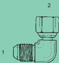
JISM-6500 - 90° (1) Male 30° Metric Komatsu Swivel (2) Fem. 30° Metric Komatsu Swivel
