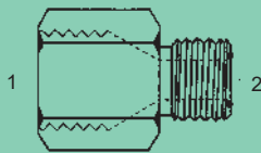
JISBP-MOFS-2406 - Str. (1) Fem. 30° BPP (Flare) (2) Male O-Ring Face Seal (SAE)
