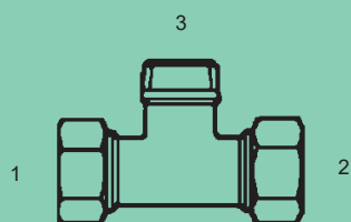
MFL-MT-2601-LL - Tee (1) (2) Male Flareless (3) Male Metric Taper Extra Light
