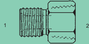
M-FP-5405 - Str. (1) Male Metric (Parallel) (2) Fem. NPT Pipe
