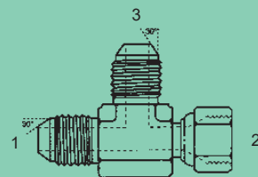
JISBP-6602 - Tee (1) (3) Male 30° BPP (Flare) (2) Fem. 30° BPP (Flare) Swivel
