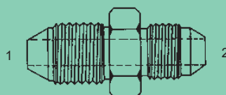
JISM-MJ-2403 - Str. (1) Male 30° Metric Komatsu Tee (2) Male 37° Tee
