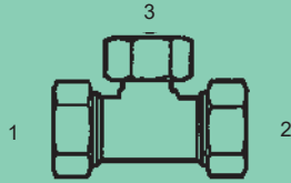
MFL-6600-H - Tee (1) (2) Male Flareless (3) Fem. Flareless Swivel Heavy
