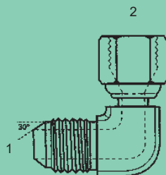
JISBP-6500 - 90° (1) Male 30° BPP (Flare) (2) Fem. 30° BPP (Flare) Swivel
