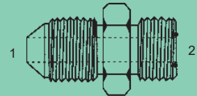
JISBP-OFS-2403 - Str. (1) Male 30° BPP (Flare) (2) Male O-Ring Face Seal (SAE)
