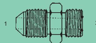
JISM-OFS-2403 - Str. (1) Male 30° Metric Komatsu Tee (2) Male O-Ring Face Seal (SAE)
