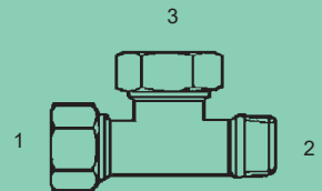
MFL-BPP-2605 - Tee (1) (3) Male Flareless (2) Male BPP w/ Cutting Face Seal Light
