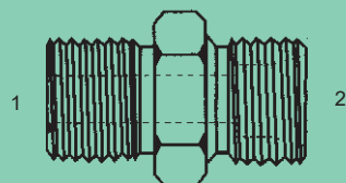
MFL-OFS-3901 - Str. (1) Male O-Ring Face Seal (2) Male Metric Dual Purpose
