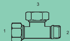
MFL-BPP-2605-H - Tee (1) (3) Male Flareless (2) Male BPP w/ Cutting Face Seal Heavy
