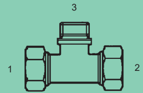
MFL-BPP-2601 - Tee (1) (2) Male Flareless (3) Male BPP w/ Cutting Face Seal Light
