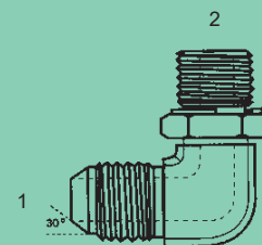
JISBP-BPP-6801-NWO - 90° (1) Male 30° BPP (Flare) (2) Male BPP Adj. O-Ring
