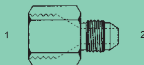
JISM-MJ-2406 - Str. (1) Fem. 30° Metric Komatsu Tee (2) Male 37° Tee
