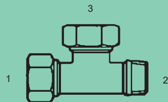
MFL-MT-2605-H - Tee (1) (3) Male Flareless (2) Male Metric Taper Heavy
