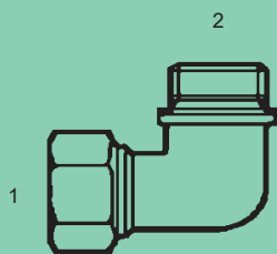
MFL-MT-2501-H - 90° (1) Male Flareless (2) Male Metric Taper Heavy
