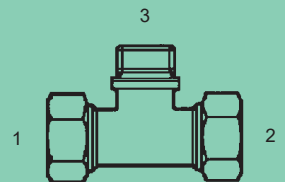
MFL-BPP-2601-H - Tee (1) (3) Male Flareless (2) Male BPP w/ Cutting Face Seal Heavy
