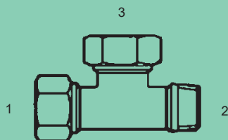
MFL-MT-2605-LL - Tee (1) (3) Male Flareless (2) Male Metric Taper Extra Light
