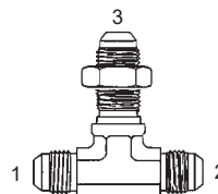
Y-2703-F-LN - Tee
