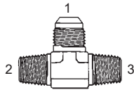
Y-2610-F - Tee
