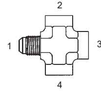
Y-2658-F - Tee
