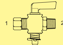
BV-304C - Str. (1) Compression (2) Male Pipe
