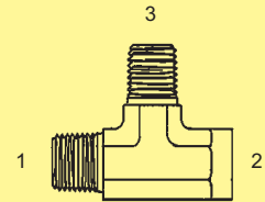
BP-5603-F - Tee (Forged) (1) (3) Male Pipe (2) Fem. Pipe
