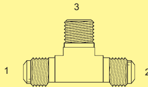
BF-2601 - Tee
