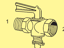
BV-402P-HP - Str. (125 PSI) (1) Male Pipe (2) Fem. Pipe
